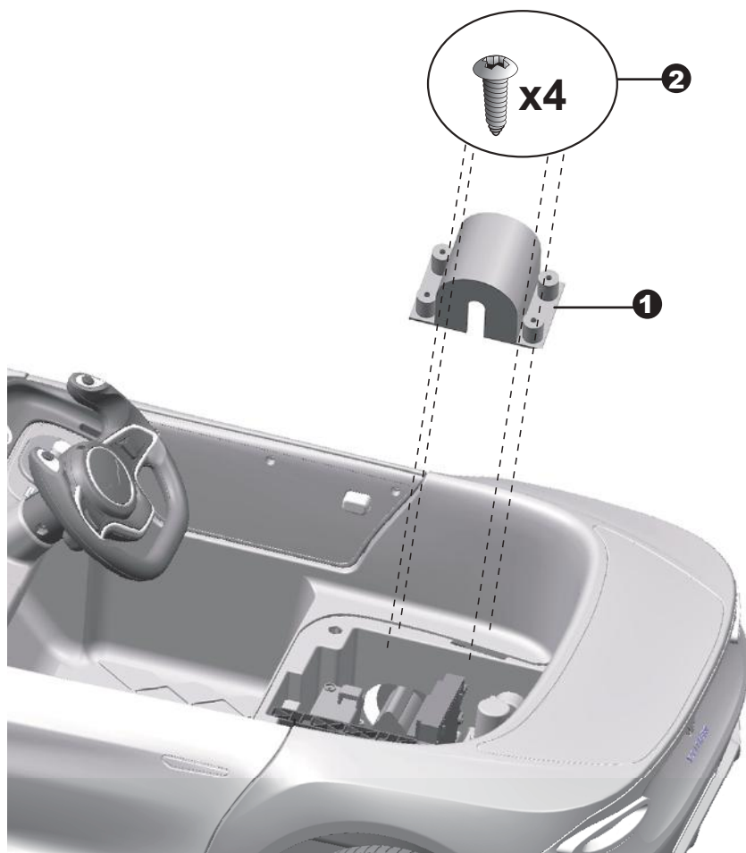
Rear View
